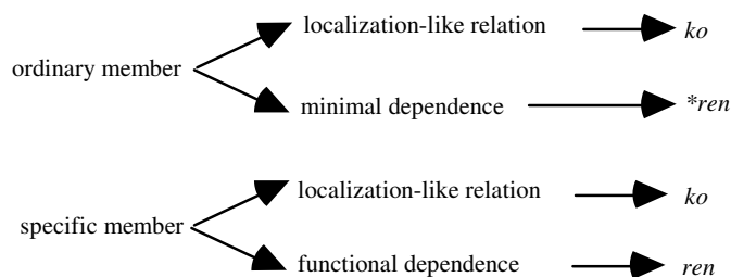
Figure 4: member-collection relations
