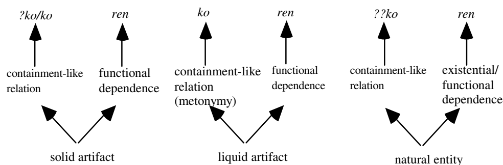
Figure 5: substance-whole relations
